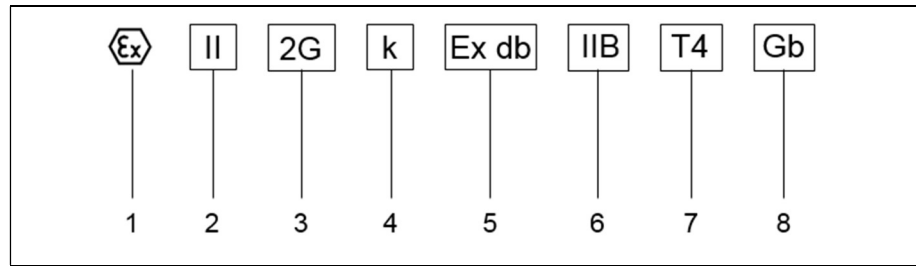
Figure 2: Explosion protection identification
