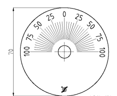
Scale 2x90° 100-0-100 Ø70 base silver, text black
